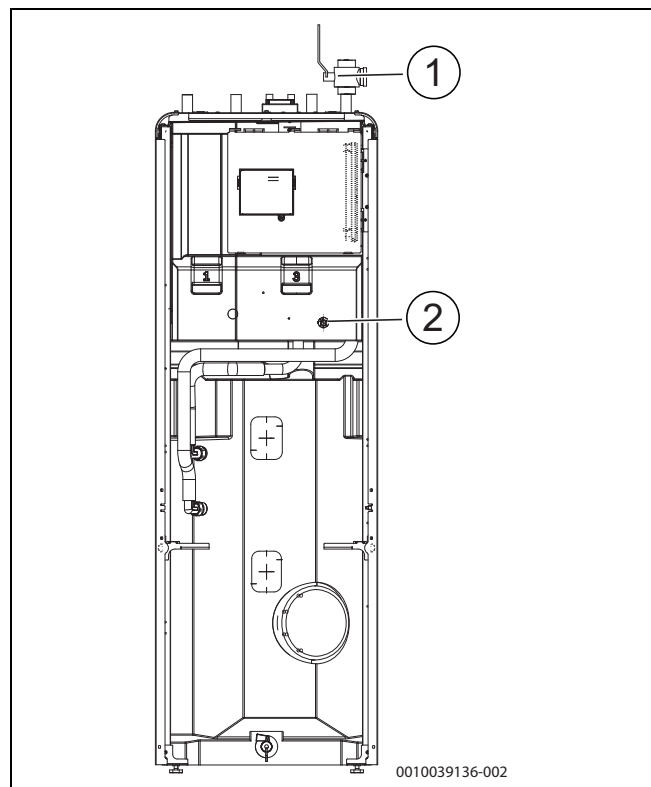
Rys. 13 Compress 5800i 12 M
