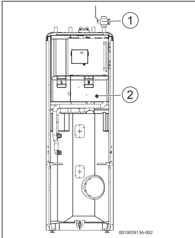
Rys. 11 Compress 5800/6800i 12 M
